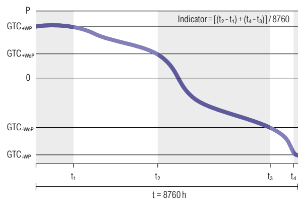
Figure 12.6: Methodology to compute indicators Deriving an estimation of security of supply improvement from the market based simulation results (a duration curve of power flow in a cross-section under study) when a project is implemented. Grid transfer capabilities with (GTC + WP, GTC - WP) and without (GTC + WoP, GTC - WoP) the project have to be known.
